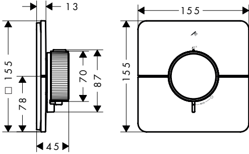
AXOR ShowerSelect ID softsquare 36758XXX
