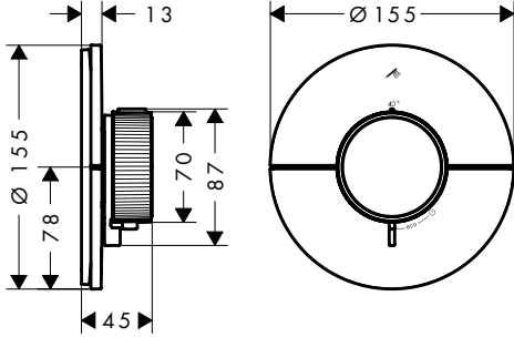
AXOR ShowerSelect ID round 36756XXX
