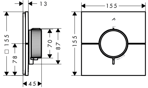
AXOR ShowerSelect ID square 36757XXX
