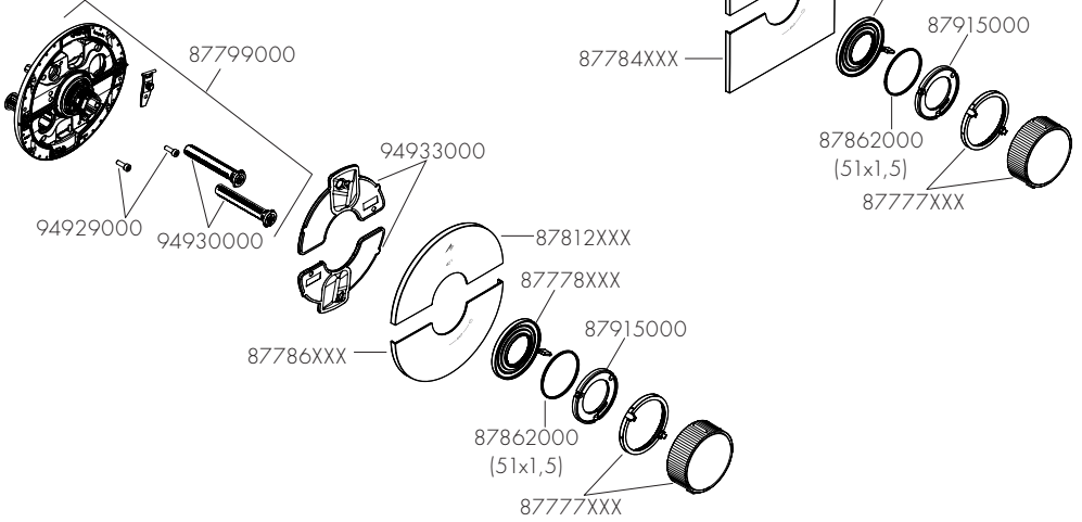
AXOR ShowerSelect ID round 36756XXX
