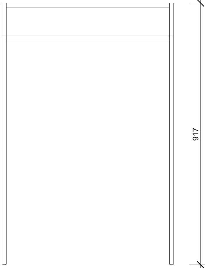
Frontansicht front view
