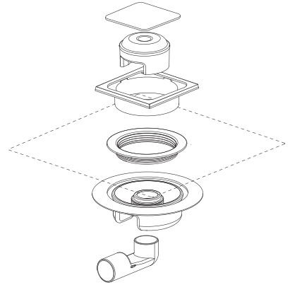
Raindrain Spot 56055800
