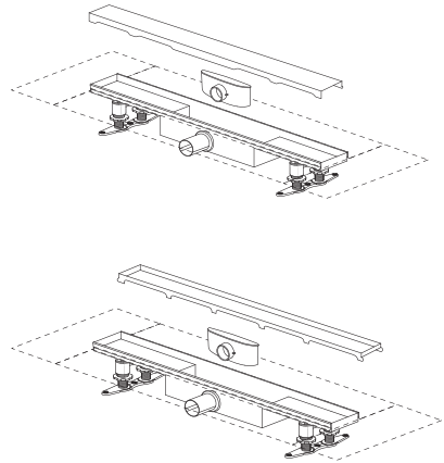
RainDrain Compact 56162800 - 56185000
