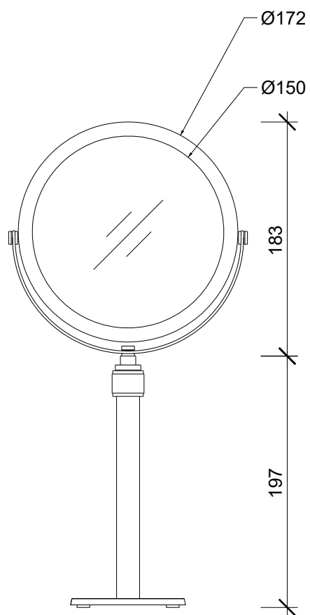
Frontansicht front view
